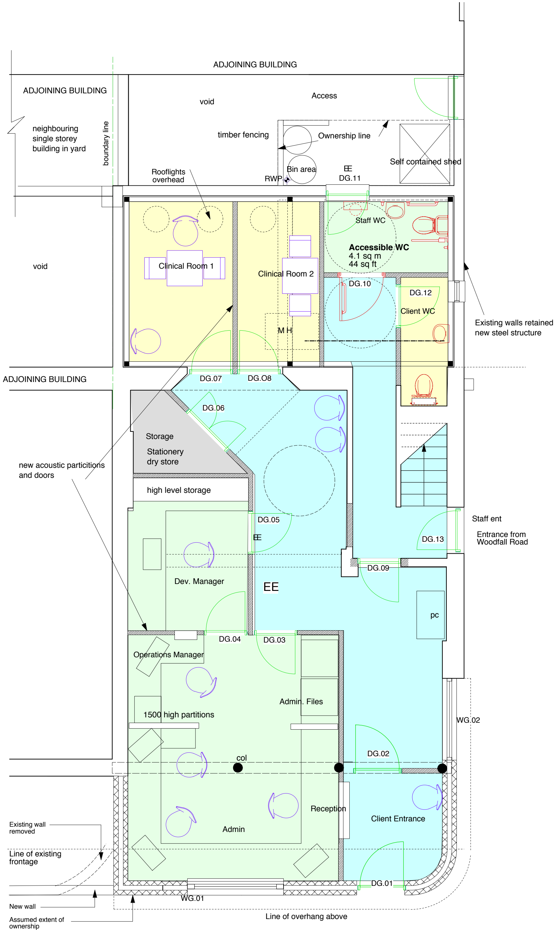
Ground Floor Furniture layout Brady Mallalieu Architects ICAP Offices 96 Moray Rd July 05
